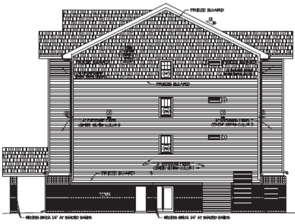
4 SOUTH ELEVATION 1/8" = 1'-0"
